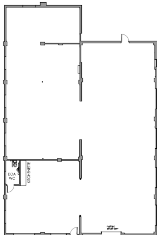
Building 2 Ground Floor Plan
